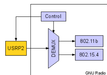
Fig. 4. Structure implemented in GNU Radio and Demux detail
