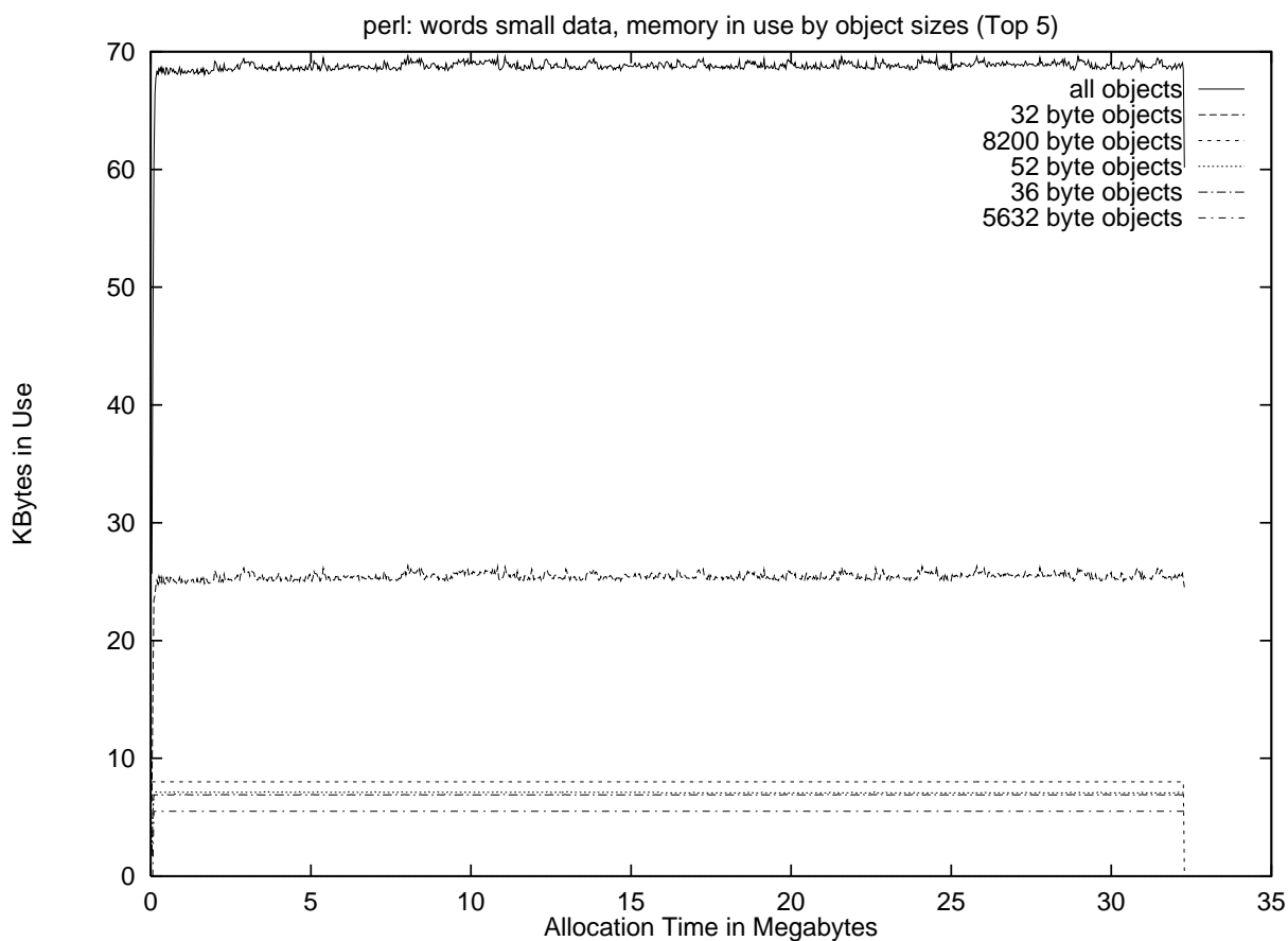
Fig. 4. Profile of memory usage in Perl running a string-processing script.
