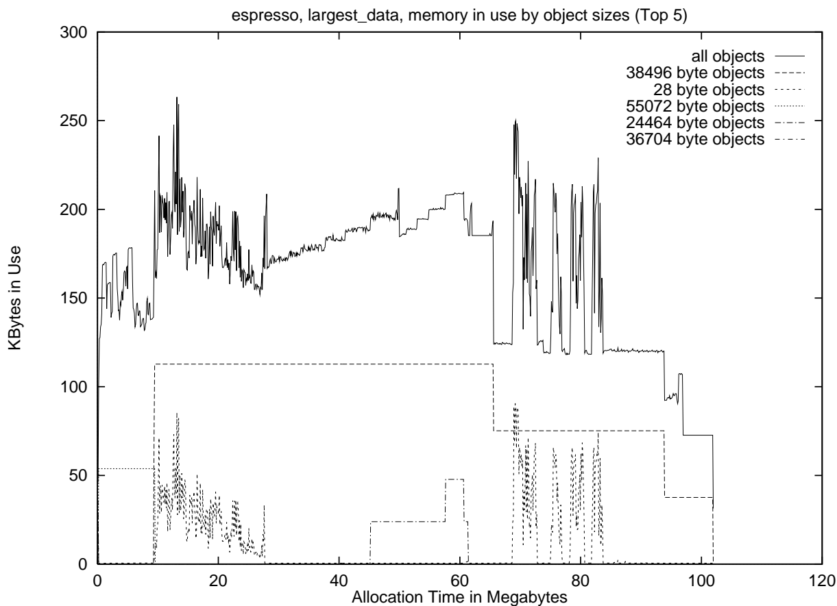
Fig. 6. Profile of memory usage in the Espresso PLA Optimizer.
